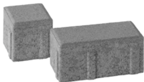
Prizma 10 Set 200 × 100 × 100 mm 100 × 100 × 100 mm
